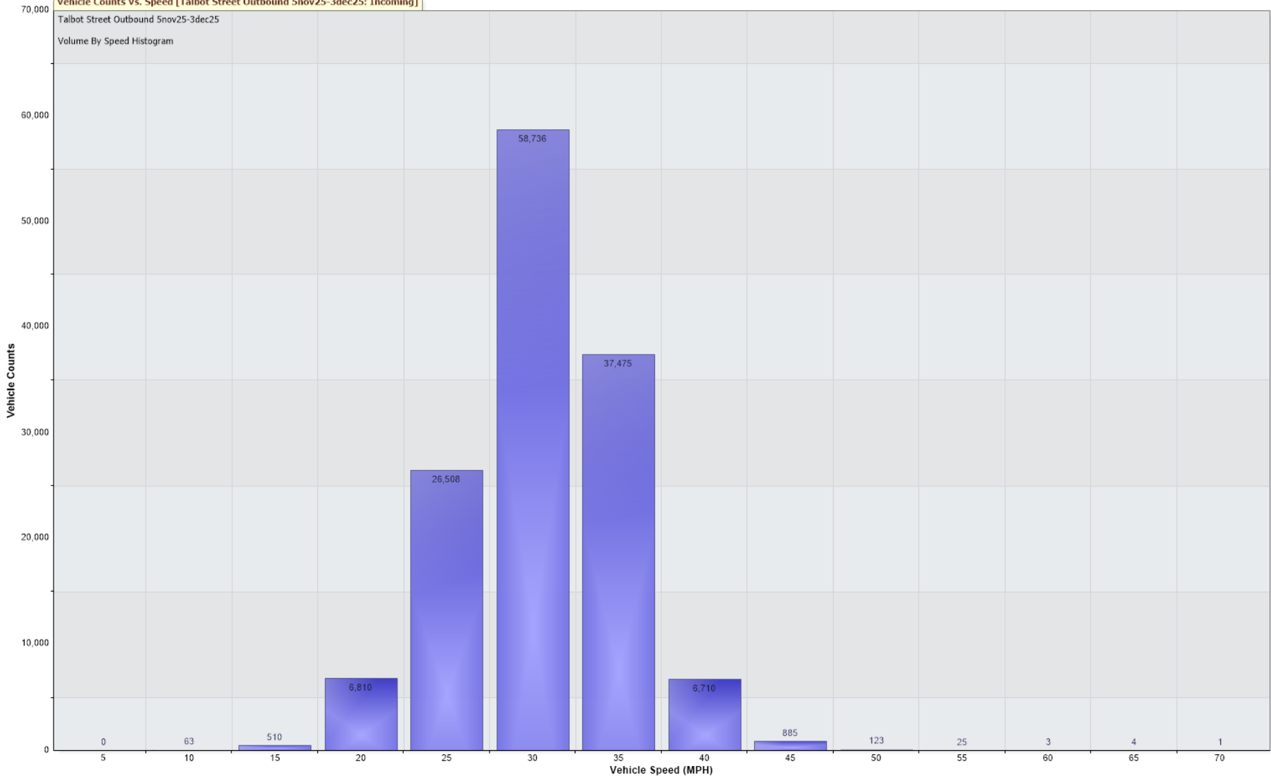
Vehicle Counts Vs. Speed [Talbot Street Outbound 5nov25-3dec25: Incoming]
