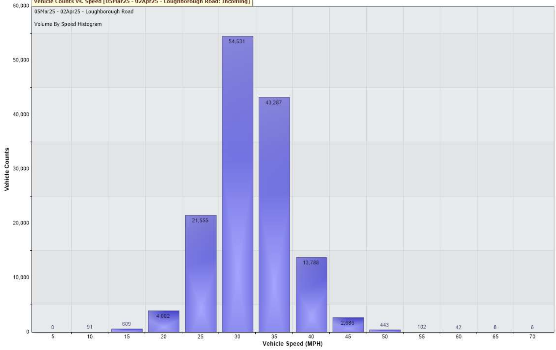
Vehicle Counts Vs. Speed [05Mar25 - 02Apr25 - Loughborough Road: Incoming]
