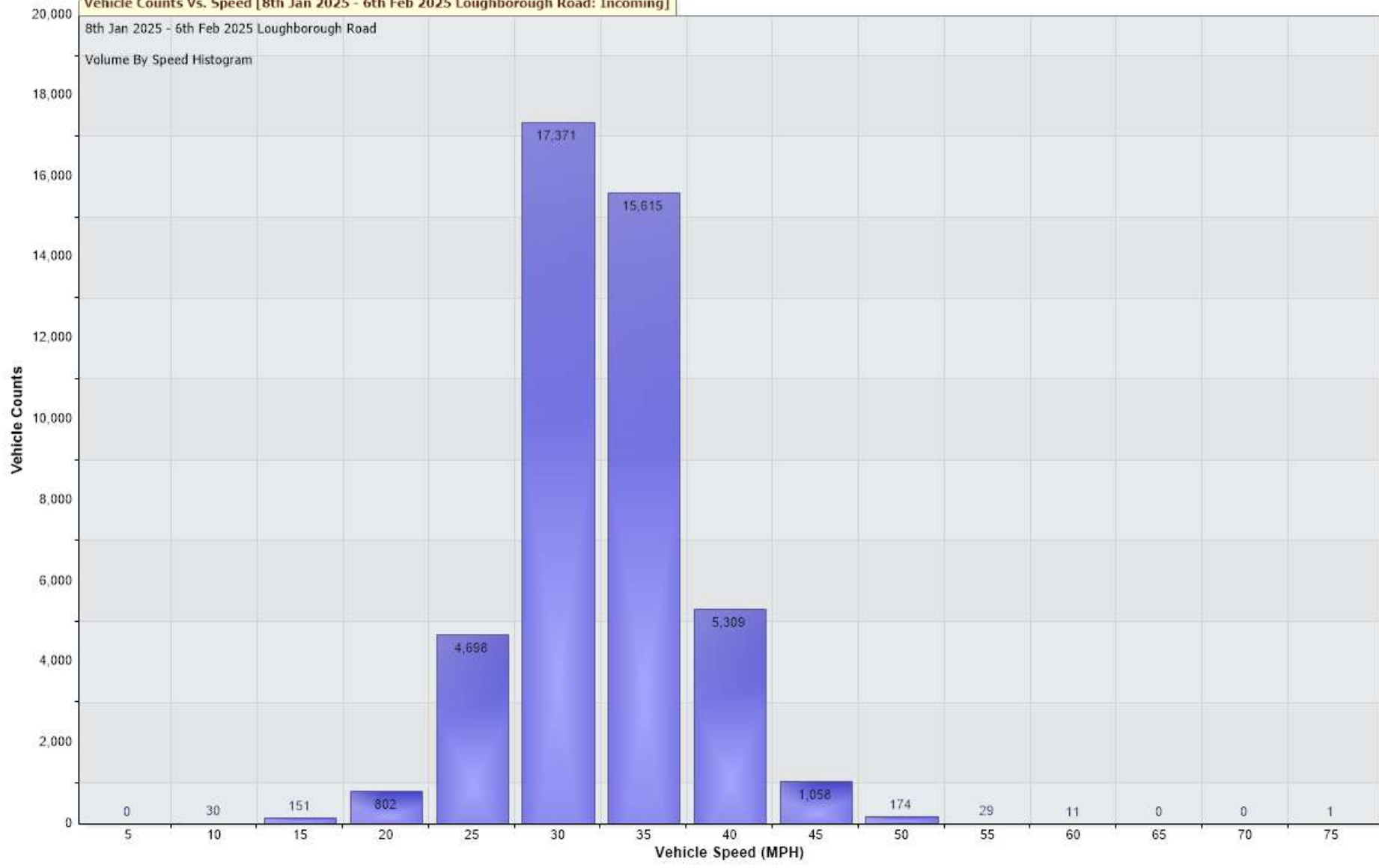
Vehicle Counts Vs. Speed [8th Jan 2025 - 6th Feb 2025 Loughborough Road: Incoming]
