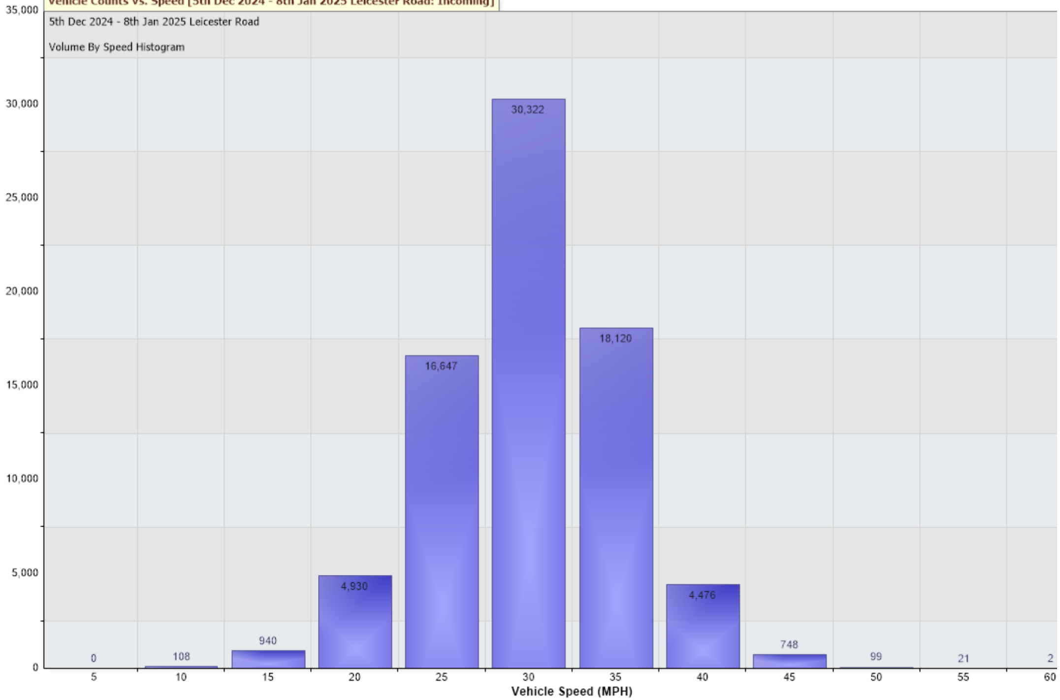
Vehicle Counts Vs. Speed [5th Dec 2024 - 8th Jan 2025 Leicester Road: Incoming]
