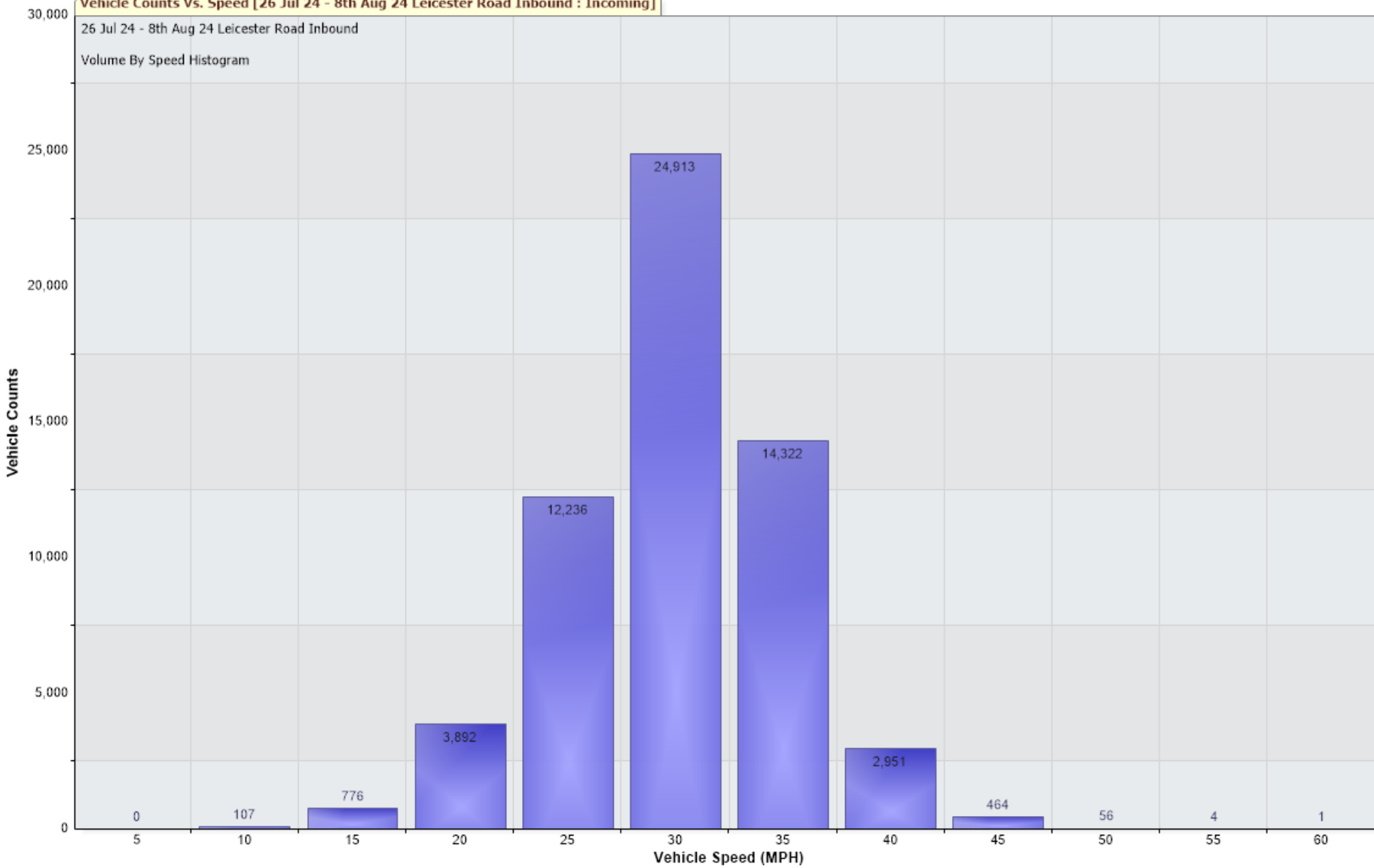
Vehicle Counts Vs. Speed [26 Jul 24 - 8th Aug 24 Leicester Road Inbound : Incoming]
