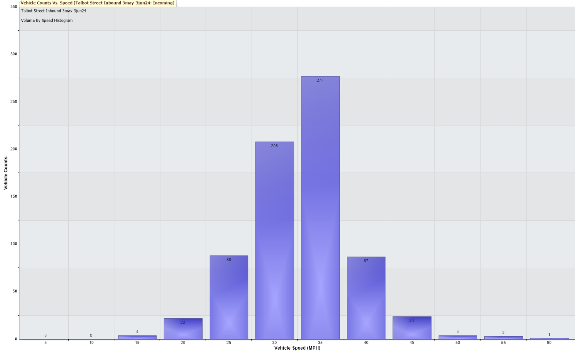
Vehicle Counts Vs. Speed [Talbot Street Inbound 3may-3jun24: Incoming]
