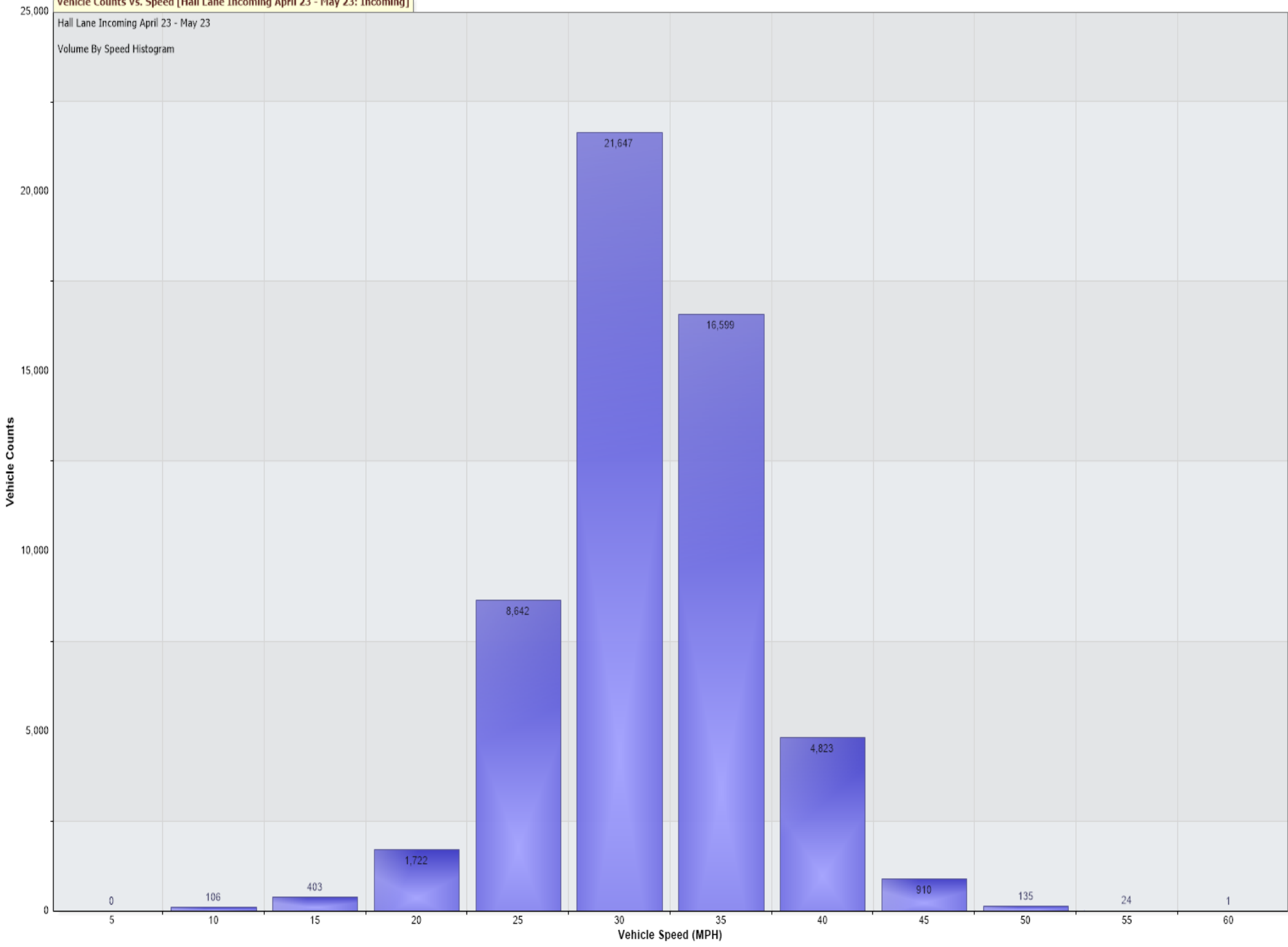
Vehicle Counts Vs. Speed [Hall Lane Incoming April 23 - May 23: Incoming]
