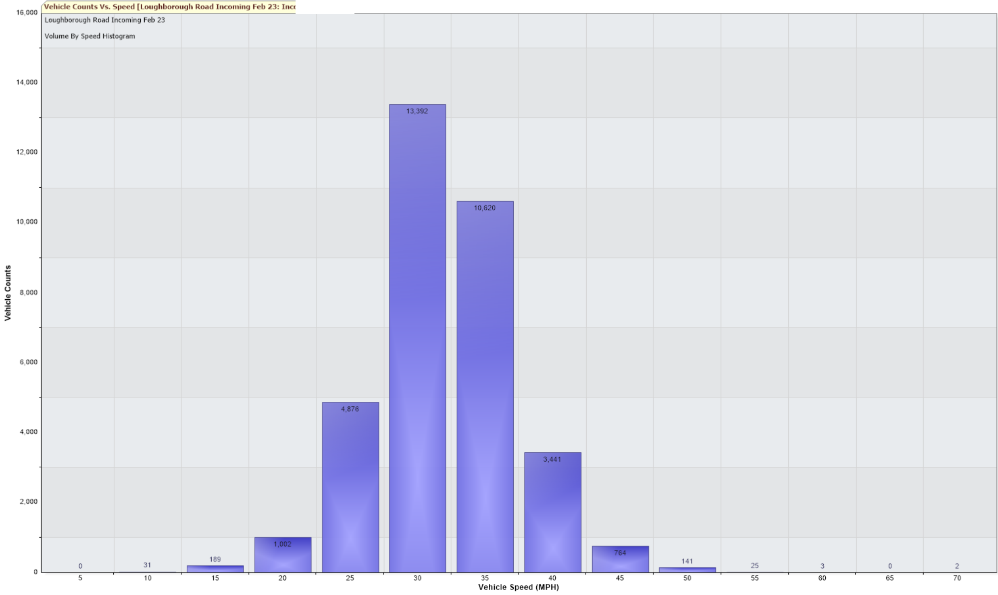
Vehicle Counts Vs. Speed [Loughborough Road Incoming Feb 23: Inco
