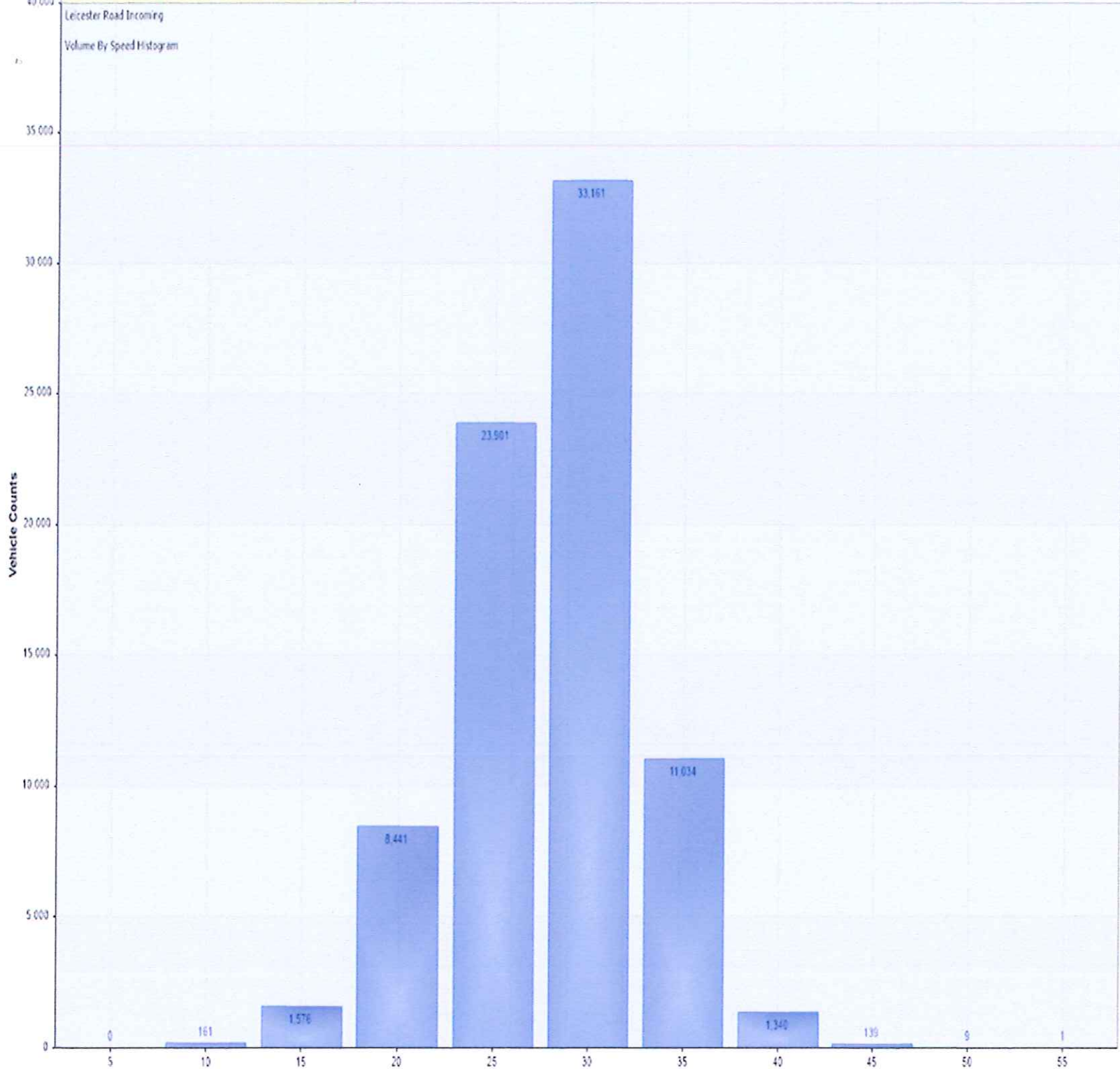
Vehicle Counts Vs. Speed [Leicester Road Incoming: Incoming]
