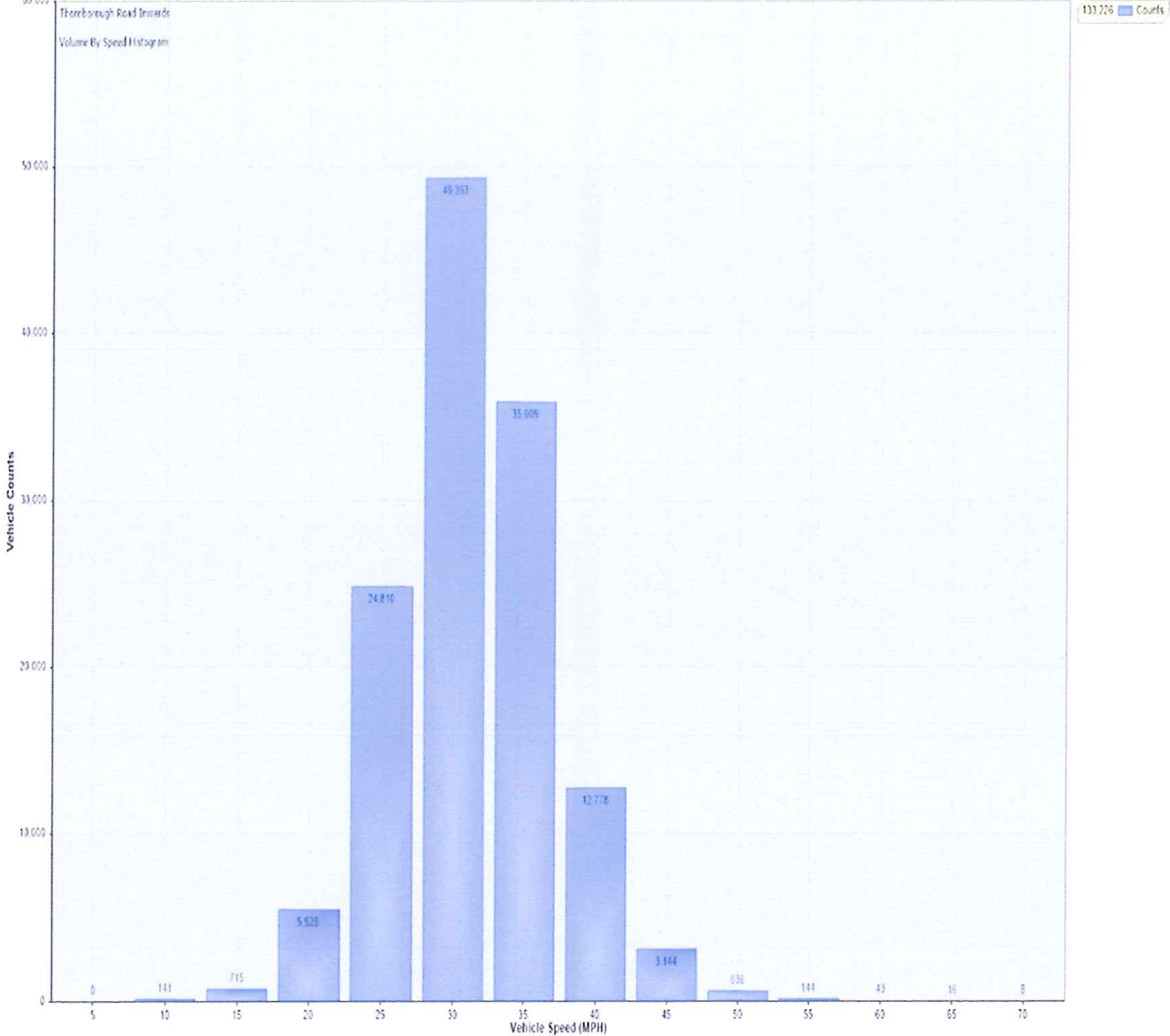
Vehicle Counts Vs. Speed [Thorough Road Inwards: Incoming]
